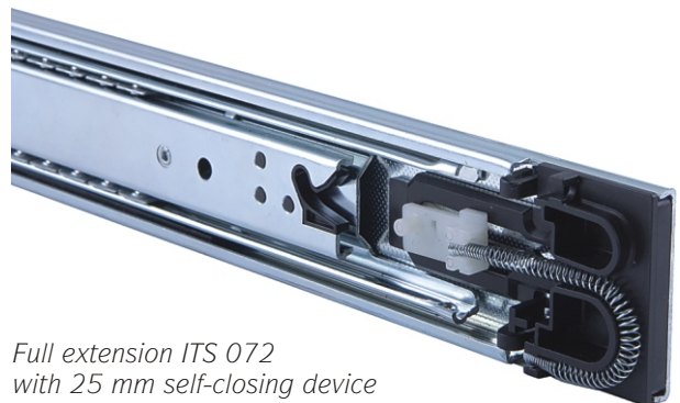
Full extension ITS 072 with 25 mm self-closing device Spring adjusted on lighter level (standard) Opening force: 7 N
